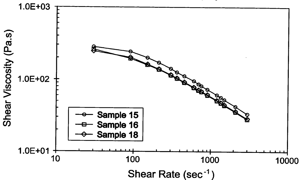
Fig. 13 Shear Viscosity of Plasticized Propylene Impact Copolymers
